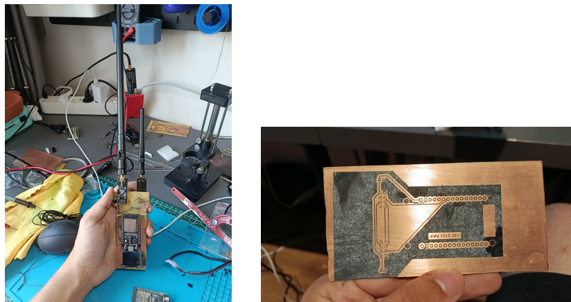
Figure 2: The first revision: toner transferred onto copper, and the same board assembled.
